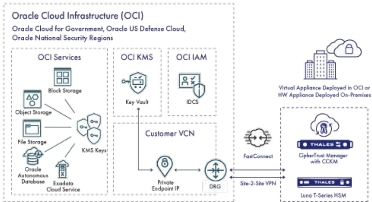
Figure 1. Deployment architecture example - CCKM hosted external to OCI
